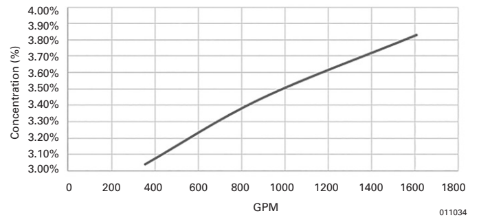
4 in. RFC with 0.522 in. Orifice
