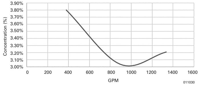
4 in. IBP with 0.480 in. Orifice
