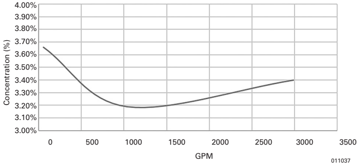
MK3 TPW 6 in. Proportioning Curve
