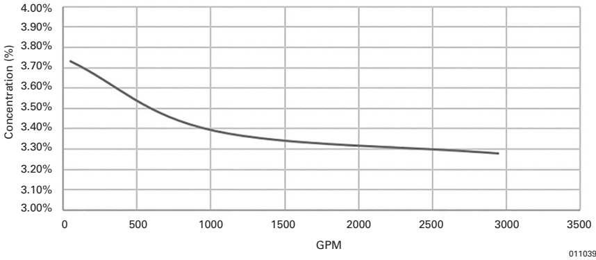
MK3 PPW 8 in. Proportioning Curve
