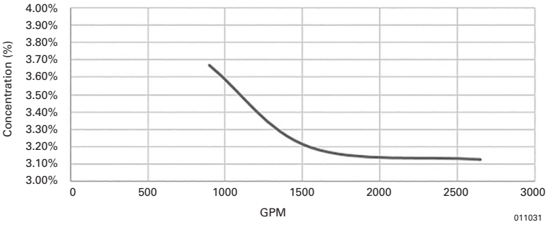
6 in. IBP with 0.648 in. Orifice
