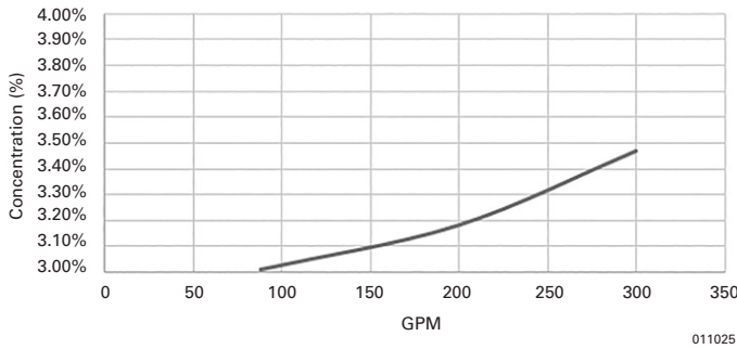
2 in. RFC with 0.203 in. Orifice
