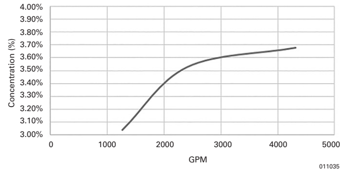
8 in. RFC with 1.200 in. Orifice
