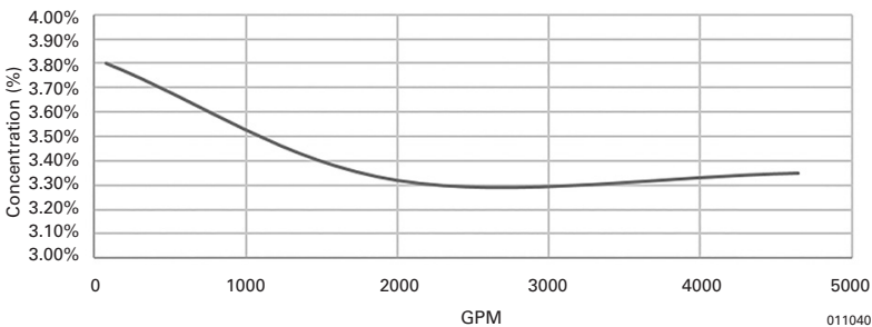
MK3 PPW 8 in. Proportioning Curve
