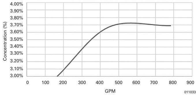
3 in. RFC with 0.405 in. Orifice
