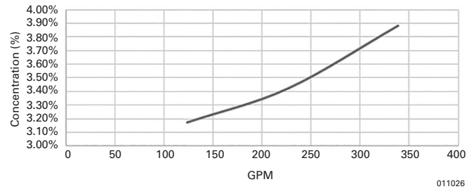
2 1/2 in. RFC with 0.268 in. Orifice
