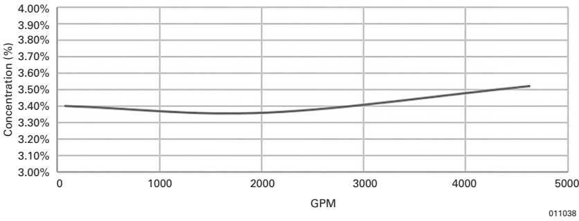
MK3 TPW 8 in. Proportioning Curve
