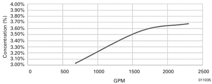
6 in. RFC with 0.810 in. Orifice
