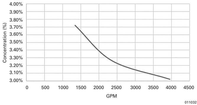
8 in. IBP with 0.914 in. Orifice
