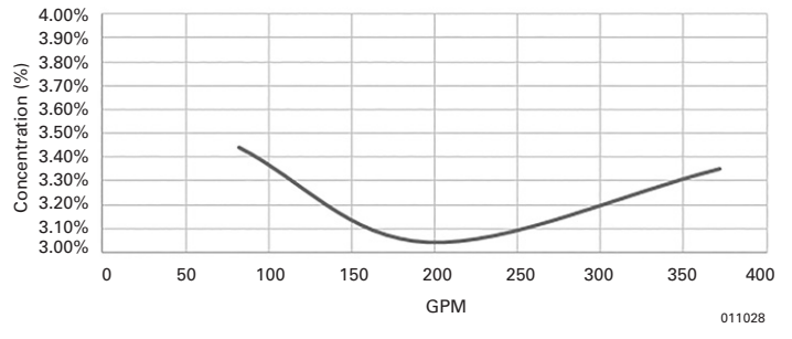
2 1/2 in. IBP with 0.242 in. Orifice
