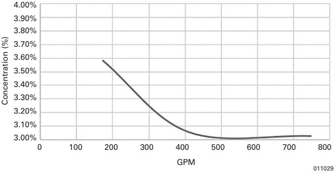
3 in. IBP with 0.347 in. Orifice
