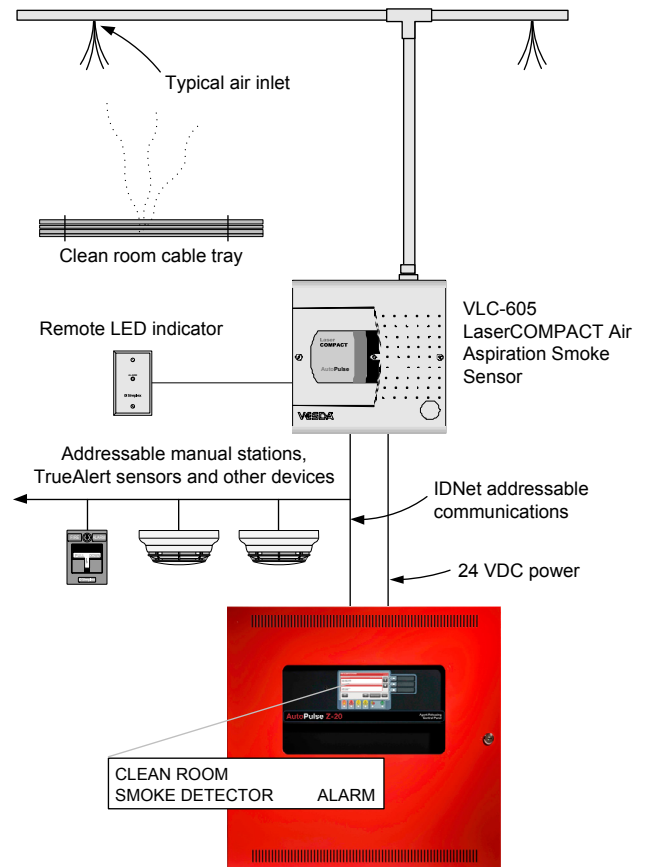
Fire Alarm Control Panel requires AUTOPULSE Z20 IDNet communications (Z20 shown for reference)
